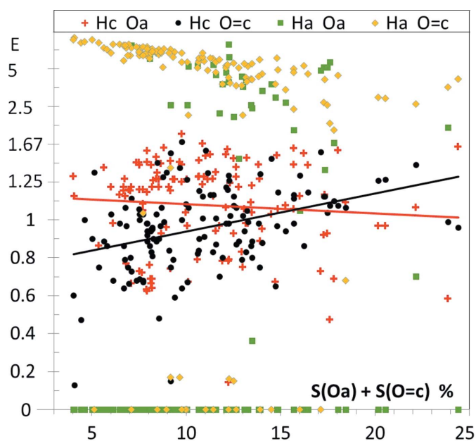
Figure 11 The enrichment of different hydrogen atom types in alcohol–carbonyl.
