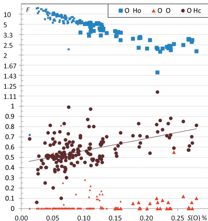
Figure 6 Contact enrichment ratios in crystals of alcohols as a function of S_O . Ho and Hc refer to the hydrogen bound to oxygen and carbon atoms, respectively. Small symbols correspond to cases where the equiprobable contacts Rxy are smaller than 2%.
