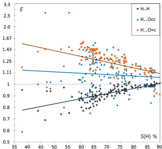
Figure 5 Contact enrichment ratios in crystals of esters as a function of S_H . Occ and O=c refer to the ether and carbonyl oxygen atom types, respectively.
