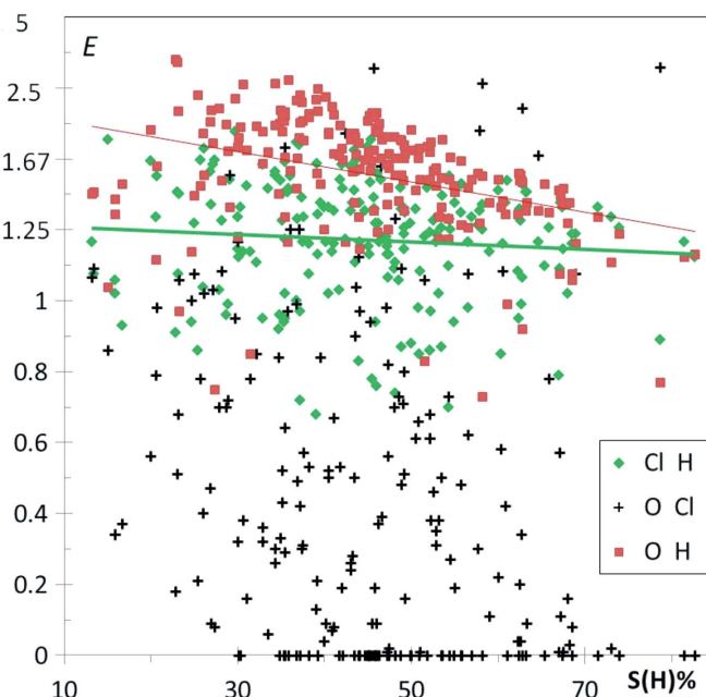
Figure 16 Enrichment of some contacts in hydrocarbons substituted with chlorine and ketone groups.
