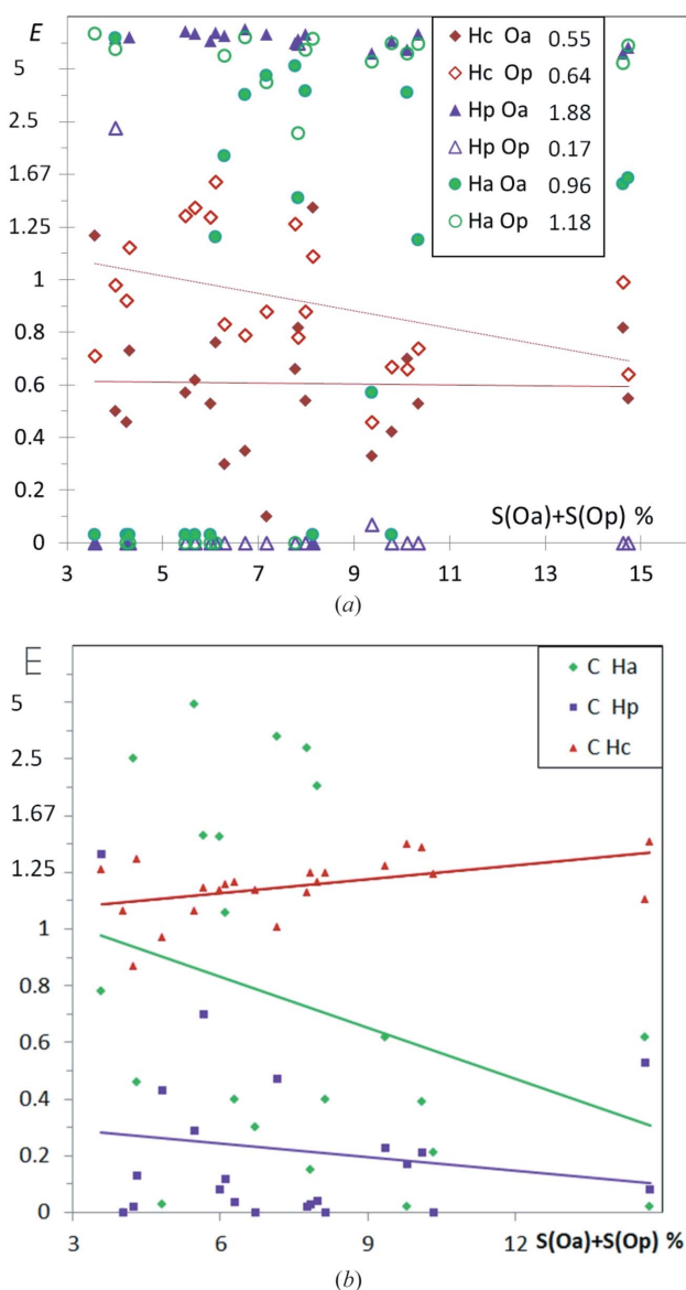
Figure 9 (a) Enrichment of six different types of O···H contacts in alcohol–phenol hydrocarbons. There are three types of hydrogen atoms, Hc, Ha and Hp and two types of oxygen atoms Oa and Op. The suffixes ‘a’ and ‘p’ refer to alcohols and phenols, respectively. The average E values are given in the legend. (b) Enrichment of different C···H contacts.
