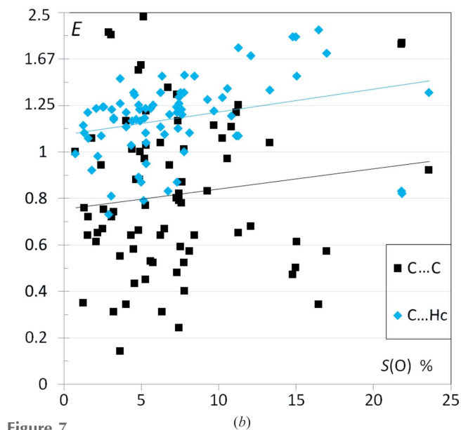
Figure 7 (a) Enrichment of O \cdots O , O \cdots Hc and O \cdots Ho contacts in phenols. Small symbols correspond to cases where the equiprobable contacts Rxy are smaller than 2%. (b) Enrichment ratios for the hydrophobic contacts types C \cdots Hc and C \cdots C .
