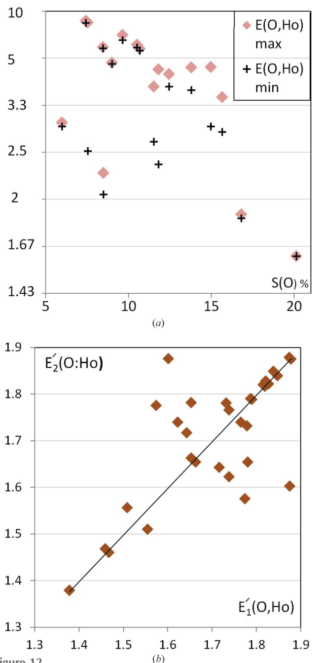
Figure 12 Enrichment of O···Ho contacts in hydroxyl–carbonyl hydrocarbons containing a dimer in the asymmetric unit. (a) The E(O, Ho) values are represented for each independent molecule as a function of oxygen content on the surface. (b) The two E' (O, Ho) values are represented as a function of each other. The ( E'_1, E'_2 ) and ( E'_2, E'_1 ) pairs are both represented in order to obtain a symmetric graph which is independent of dimer #1 and #2 attributions.
