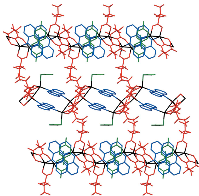
Figure 3 Stacking of one-dimensional coordination polymer chains in 1-pxyl , [\text{Ag}_4(\text{O}_2\text{C}(\text{CF}_2)_2\text{CF}_3)_4(\text{phenazine})_2(p\text{-xylene})_2] . H atoms omitted for clarity. Colours are as in Fig. 1. 1-mxyl is isostructural with 1-pxyl .
