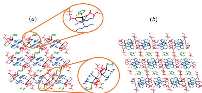
Figure 2 Crystal structure of [\text{Ag}_4(\text{O}_2\text{C}(\text{CF}_2)_2\text{CF}_3)_4(\text{phenazine})_2(\text{toluene})] \cdot 2(\text{toluene}) ( 1-tol-tol ) shown (a) in the ab plane, highlighting the \mu\text{-}\eta^1, \eta^1 bridging toluene molecules (expansions showing the silver carboxylate dimer and the tetramers; only one of the two toluene orientations is shown in the expansions) and (b) in the bc plane, highlighting the non-coordinated toluene solvent between two-dimensional layers of 1-tol-tol . Silver ions shown in black, heptafluorobutanoate in red, phenazine in blue and toluene in green. H atoms omitted for clarity.
